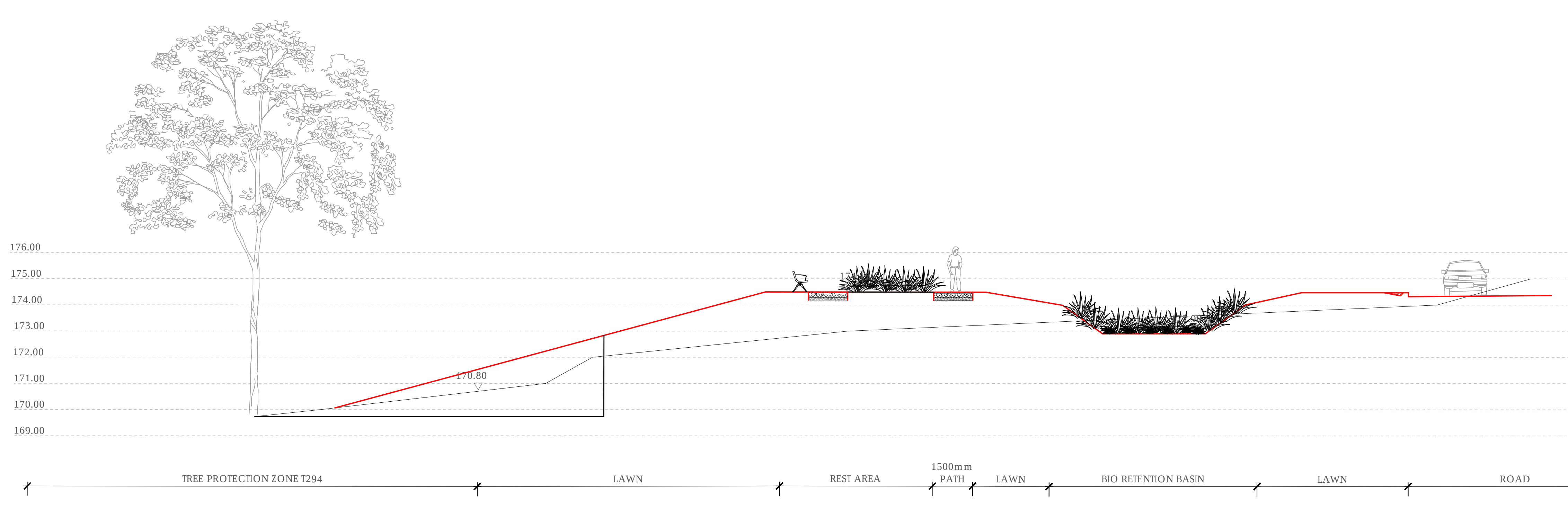
01 SECTION ONE SCALE 1:100
