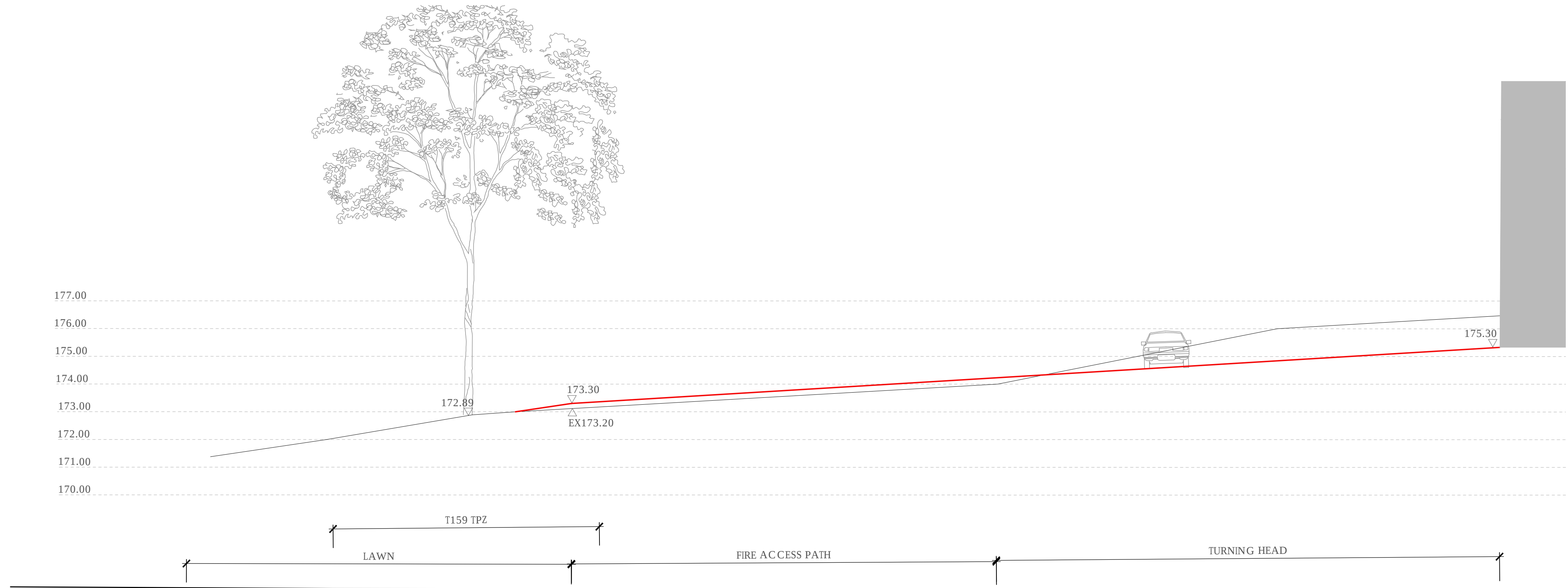
01 SECTION THREE SCALE 1:100
