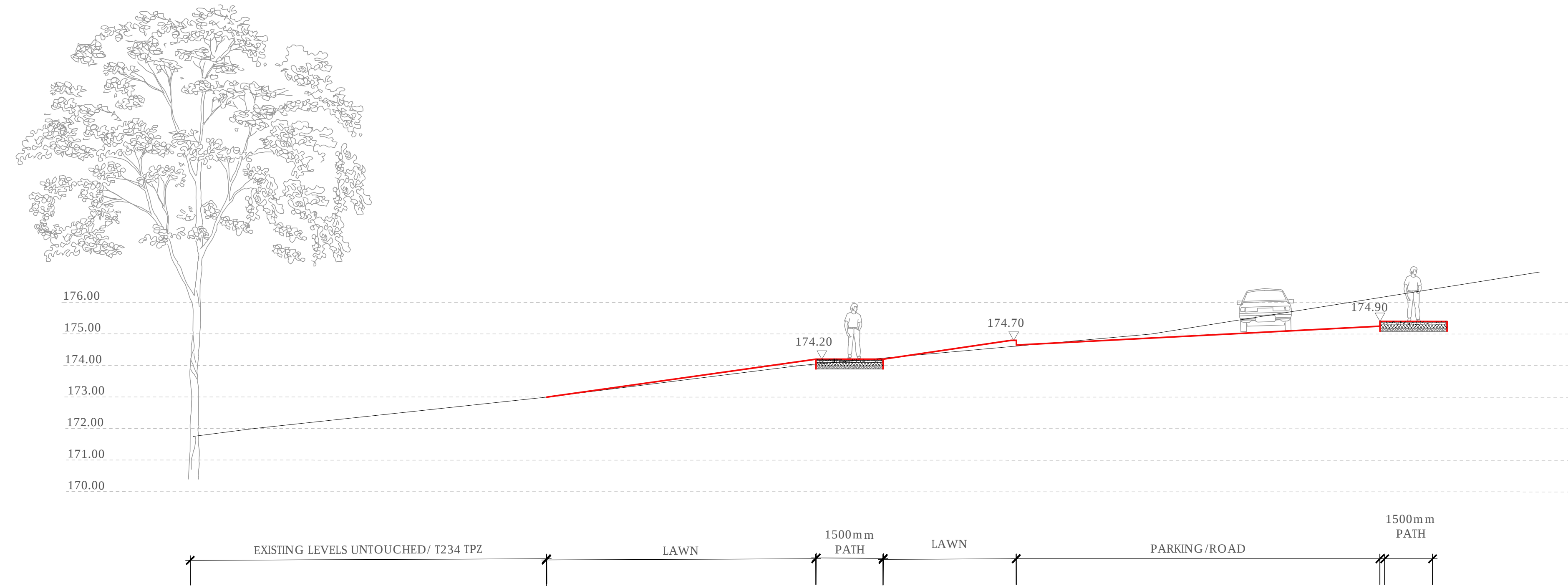
02 SECTION TWO SCALE 1:100
